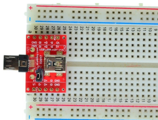
Figure 2: Example of connecting the USB-uBM-mBF-V1A on a breadboard (Note: This picture only shows the pins spacing, actual use may not be used on a breadboard)
